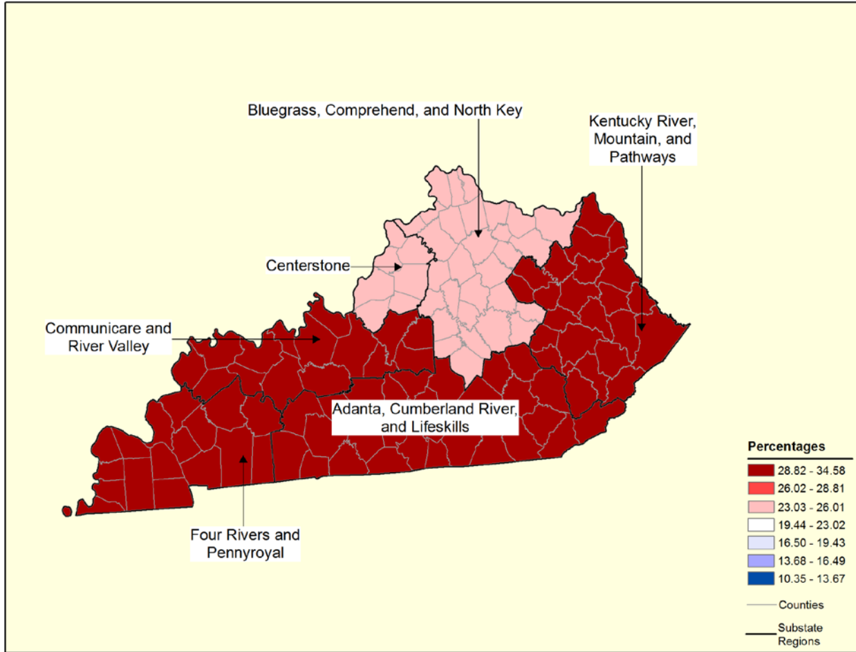
Figure 18.9 Cigarette Use in the Past Month among Individuals Aged 12 or Older in Kentucky, by Substate Region: Percentages, Annual Averages Based on 2014, 2015, and 2016 NSDUHs
